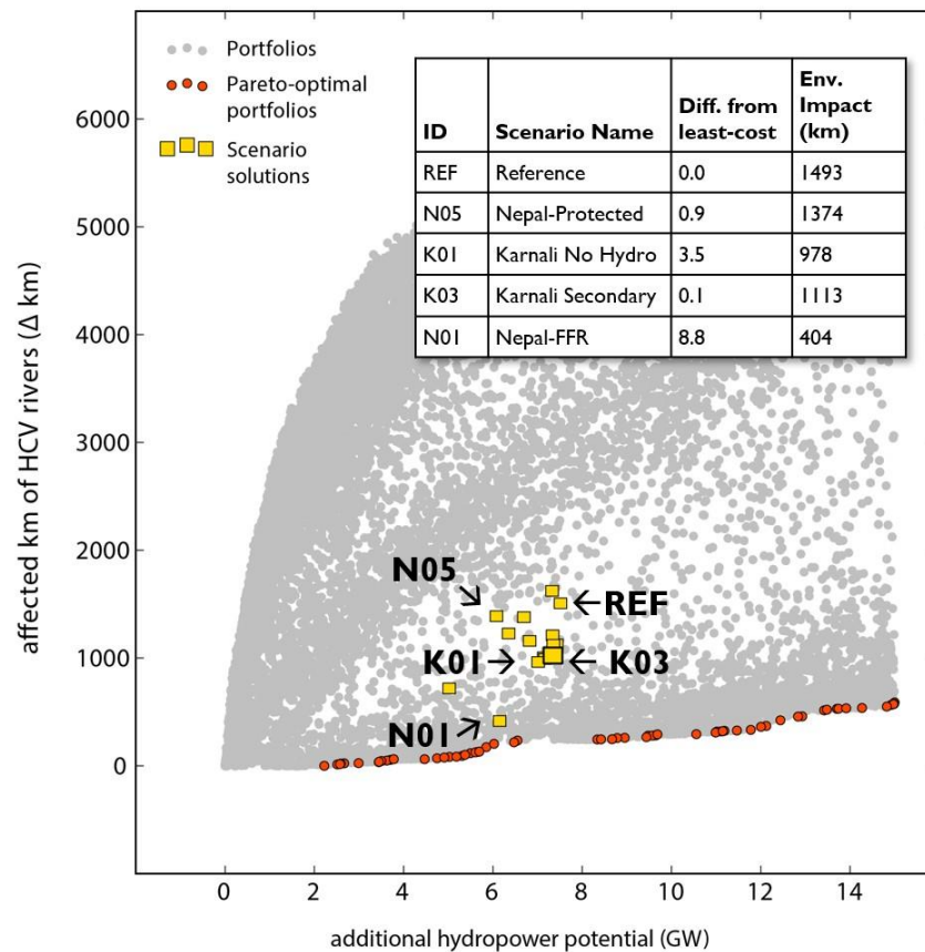
Figure 20: Least-cost environmental scenarios from the SWITCH energy options model evaluated in the SSP context
